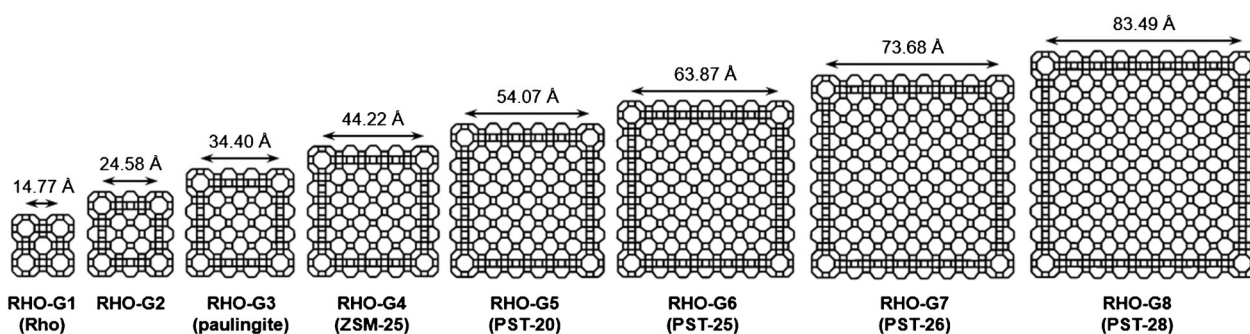
Figure 1. Framework representations of cross-sections (circa 12 Å thick) of RHO-G1 to RHO-G8 in the RHO family of zeolites. Structures RHO-G7 and RHO-G8 were predicted and then synthesized in this work.
